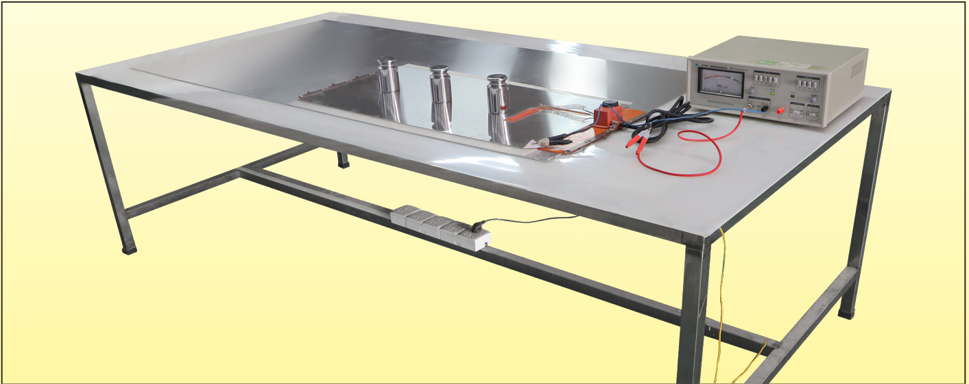
Device for measuring the insulation resistance. The measured values are always greater than 0.1Gohm
