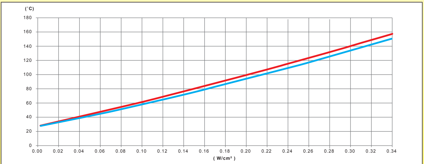
Variation, as a function of the power in W/cm² of the silicone heating ribbon, of the wall temperature of an empty stainless-steel tube, thermally insulated by 20mm of PVC-NBR foam
