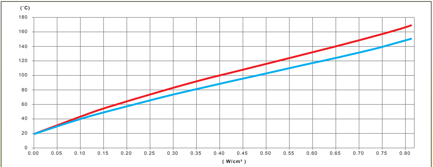
Variation, as a function of the power in W/cm² of the silicone heating ribbon, of the wall temperature of an empty, non-thermally insulated stainless steel tube
