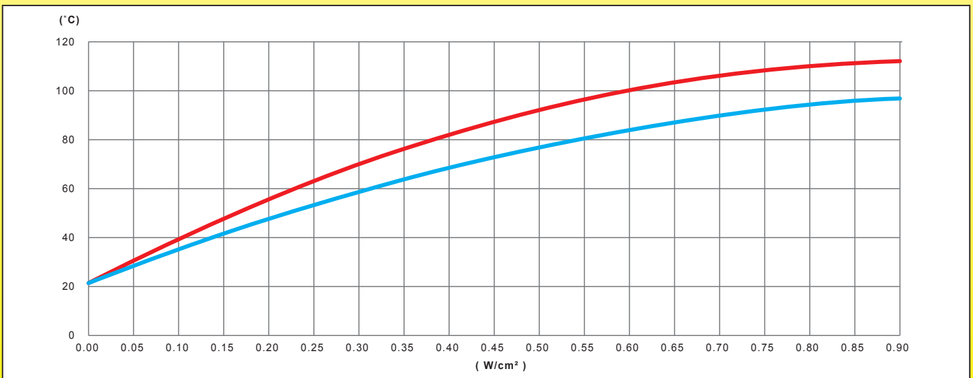
Variation, as a function of the power in W/cm² of the silicone heating ribbon, of the wall temperature of a stainless-steel tube, filled with non-circulated water, no-thermally insulated
