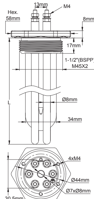
With 1"1/2 BSPP or M45x2 fitting
