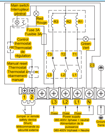
Temperature control thermostat and manual reset thermostat
