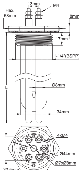
With 1"1/4 BSPP fitting
