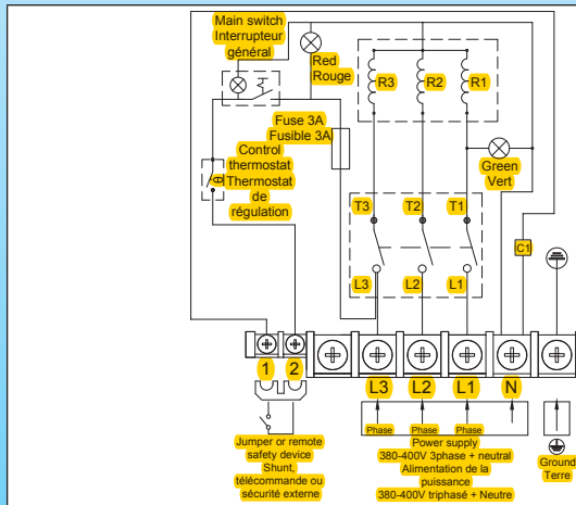
Temperature control thermostat
