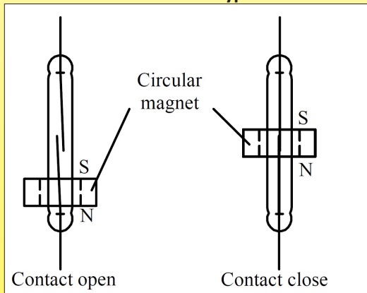
A1: Vertical type
