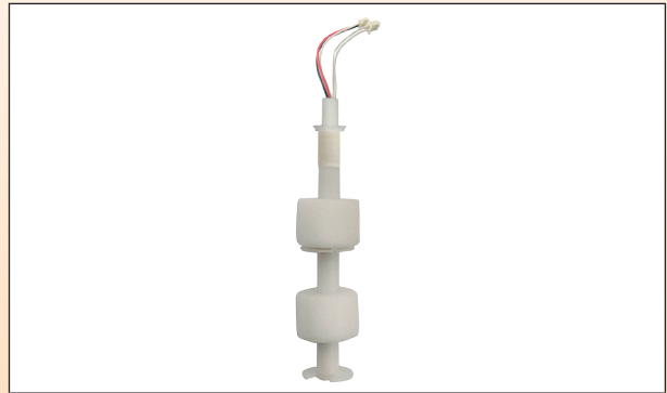
Vertical mounting, two EPS foam floats
